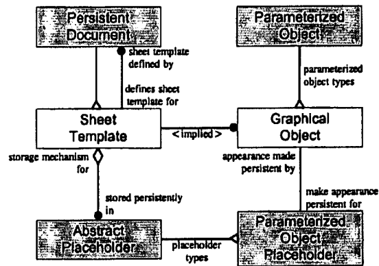
Figure 36 - Sheet Templates Object Model
